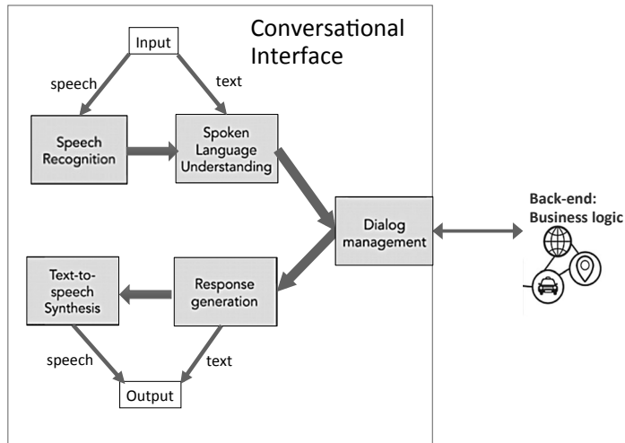
Figure 1 - Typical architecture of a conversational interface
