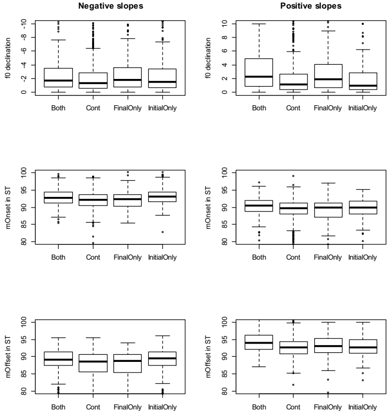
Figure 3: Boxplots for f0 midline slopes (upper tracks), initial f0 value of the midline (middle tracks), final f0 value of the midline (lower tracks) for different communicative events. Data are split into negative f0 slopes <0 (left graphs) and positive ones f0 slope >0 (right graphs).
